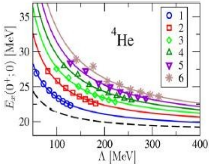
Fig. 2. Dependence of the first (0^+; 0) excitation energy in ^4\text{He} on the ultraviolet momentum cutoff \Lambda . For each frequency \hbar\omega , given in the legend in MeV, we interpolate the direct results (discrete symbols) with a 1/\Lambda dependence (continuous curves). The dashed curve marks the limit \hbar\omega \rightarrow 0 .
