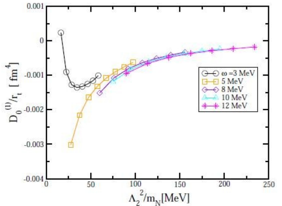
FIG. 13: Three-nucleon coupling constants as function of \Lambda_2^2/m_N , for different values of \omega : D_0^{(0)}\Lambda_2^2/m_N (left panel) and D_0^{(1)}/r_t (right panel).
