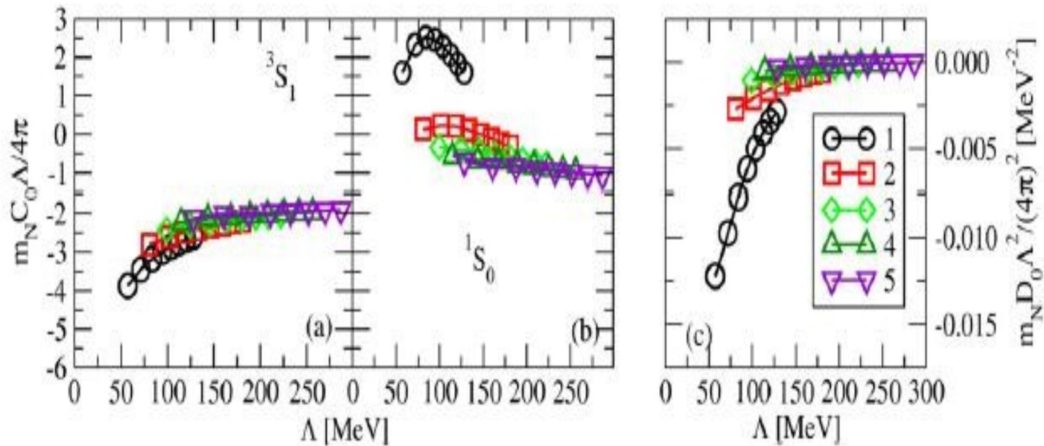
Fig. 1. Running of the scaled NN and NNN coupling constants with the ultraviolet cutoff \Lambda at various frequencies \hbar\omega given in the legend in MeV: (a) m_N \Lambda C_0^1 / 4\pi ; (b) m_N \Lambda C_0^0 / 4\pi ; and (c) m_N \Lambda^2 D_0 / (4\pi)^2 .
