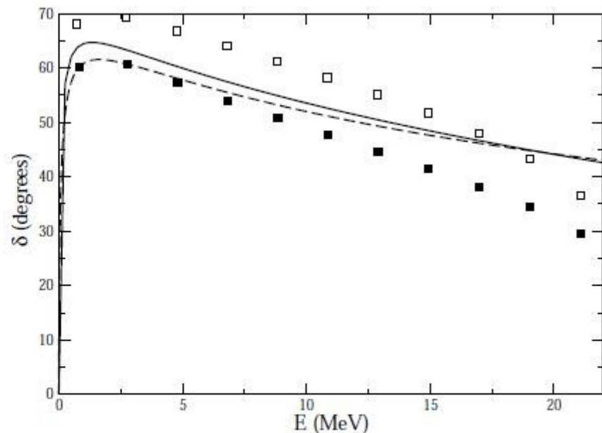
FIG. 5: Phase shifts for the two-nucleon system at \omega = 1 MeV and N_{max} = 20 as a function of the relative energy: ^3S_1 (left panel) and ^1S_0 (right panel). EFT results at LO (NLO) are marked by empty (filled) squares; the ERE up to the effective range is indicated by a dashed line; and the Nijmegen np PSA [20] by a solid line.
