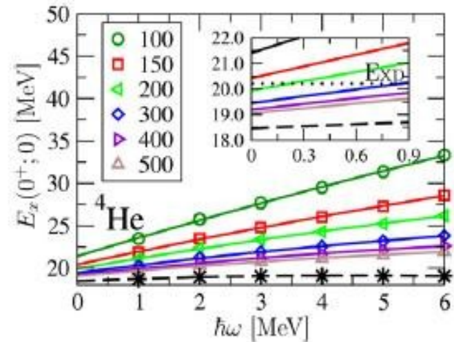
Fig. 3. Dependence of the first (0^+; 0) excitation energy in ^4\text{He} on the infrared energy cutoff \hbar\omega . For each ultraviolet cutoff \Lambda , given in the legend in MeV, we interpolate as described in the text. The results marked with star symbols are obtained in the limit \Lambda \rightarrow \infty . In the insert we show the variation around the origin, compared to the experimental value.
