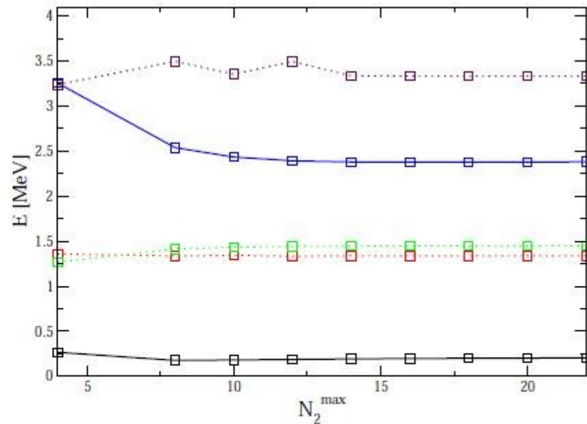
FIG. 8: Lowest energies of the trapped three-nucleon system with T = 1/2 , J^\pi = 3/2^+ as a function of N_2^{max} , for \omega = 1 MeV: LO (left panel) and NLO (right panel). The ground state and the third excited state (full lines) correspond to neutron-deuteron scattering within the trap in the L = 0 , S = 3/2 channel, whereas the other states shown correspond to different L , S configurations.
