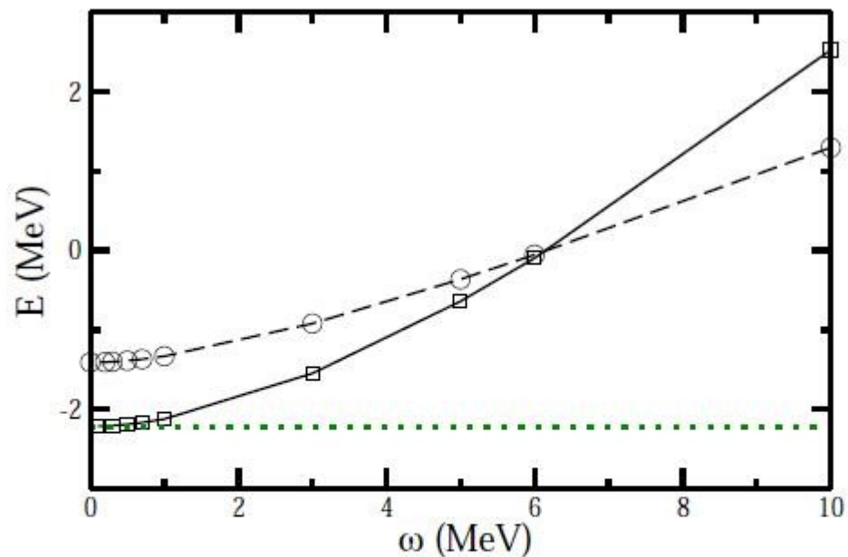
FIG. 1: Ground-state energy of the trapped two-nucleon system in the ^3S_1 channel (deuteron in the trap) as a function of the frequency \omega . The energy at LO (NLO) is given by the dashed (solid) line. For small values of \omega , the energy converges to the value in free space, which is, at NLO, indicated by the dotted line.
