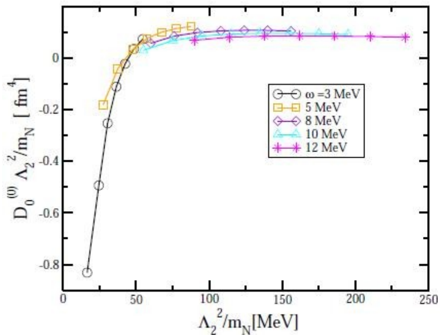
FIG. 13: Three-nucleon coupling constants as function of \Lambda_2^2/m_N , for different values of \omega : D_0^{(0)}\Lambda_2^2/m_N (left panel) and D_0^{(1)}/r_t (right panel).
