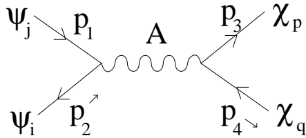
Figure 2: The Feynman diagram for \psi\bar{\psi} \rightarrow \chi\bar{\chi} .
