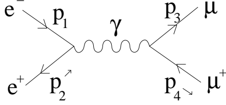
Figure 1: Leading Feynman diagram for e^+e^- \rightarrow \mu^+\mu^- .
